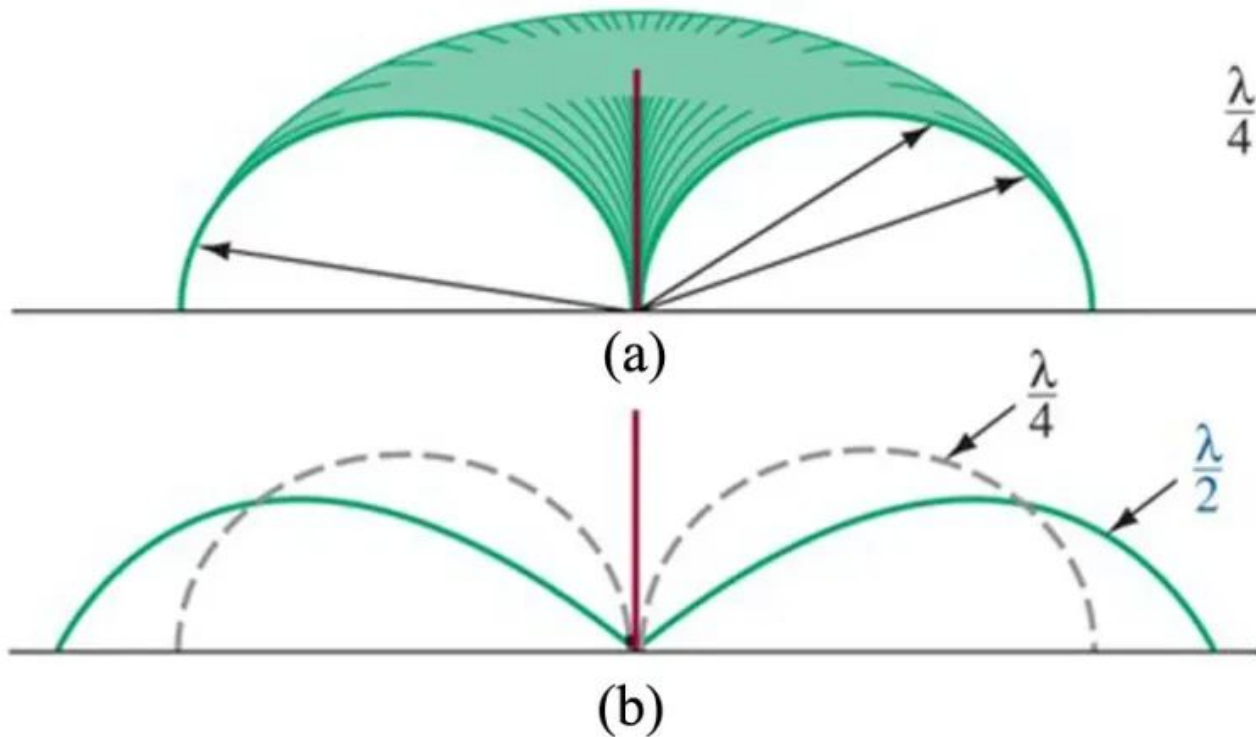
Figure 3: Vertical antenna radiation patterns
